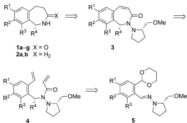
Scheme 1. Retrosynthetic analysis of chiral benzazepin(on)es.
