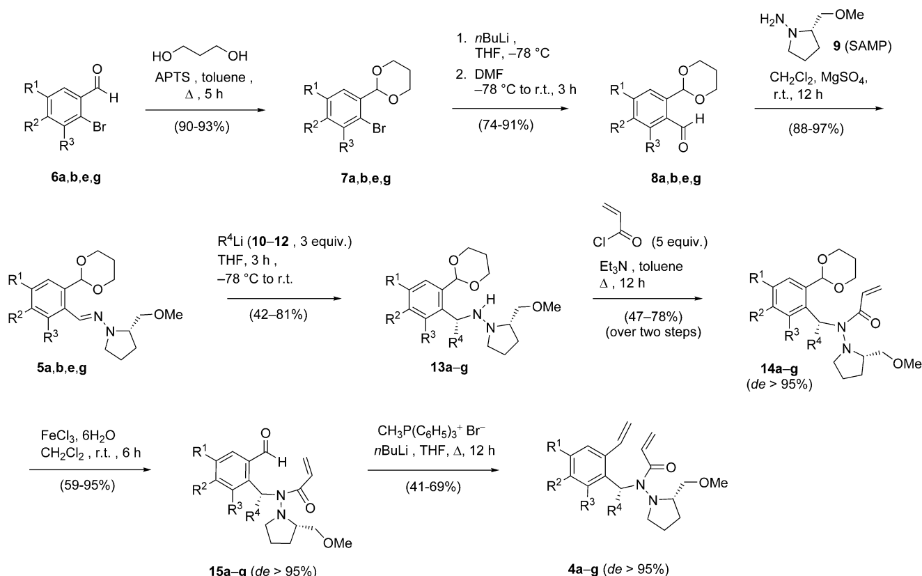
Scheme 2. Synthesis of the styrenic enehydrazides 4a-g .
