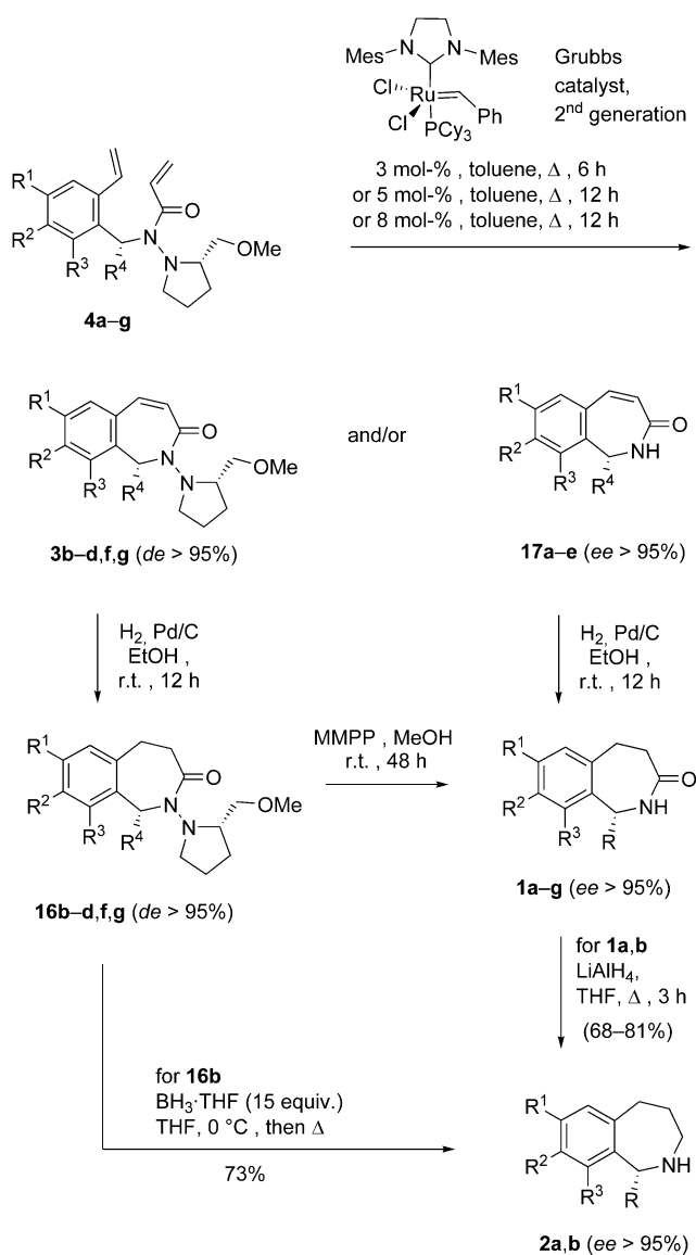
Scheme 3. Asymmetric synthesis of benzazepinones 1a–g and benzazepines 2a,b .
